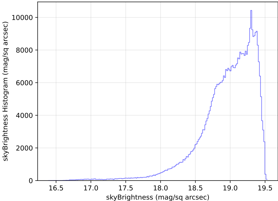
too_100_4v3.4_10yrs WFD z band: skyBrightness Histogram
