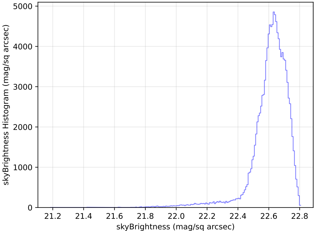
too_100_4v3.4_10yrs WFD u band: skyBrightness Histogram
