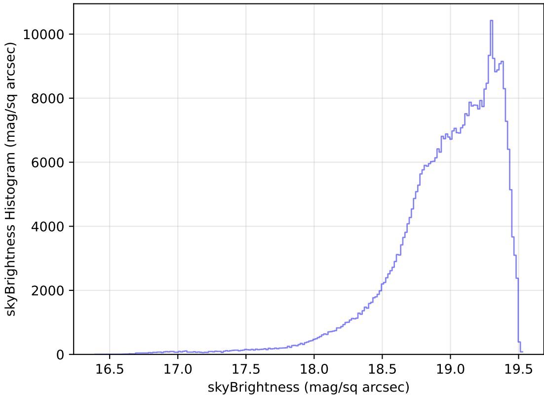
too_100_4v3.4_10yrs All sky z band: skyBrightness Histogram
