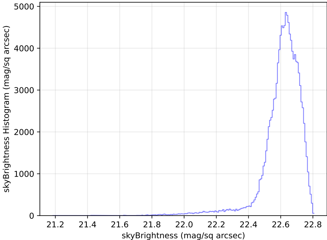
too_100_4v3.4_10yrs All sky u band: skyBrightness Histogram
