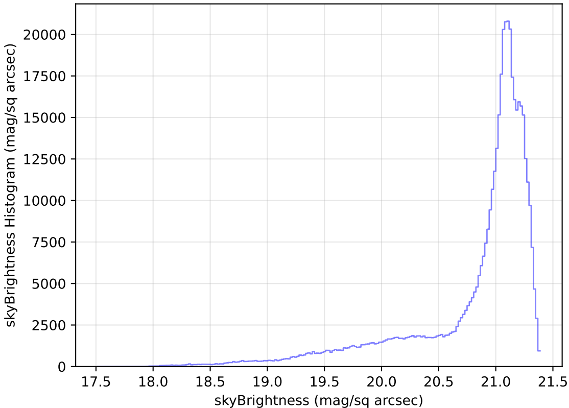
too_100_4v3.4_10yrs All sky r band: skyBrightness Histogram
