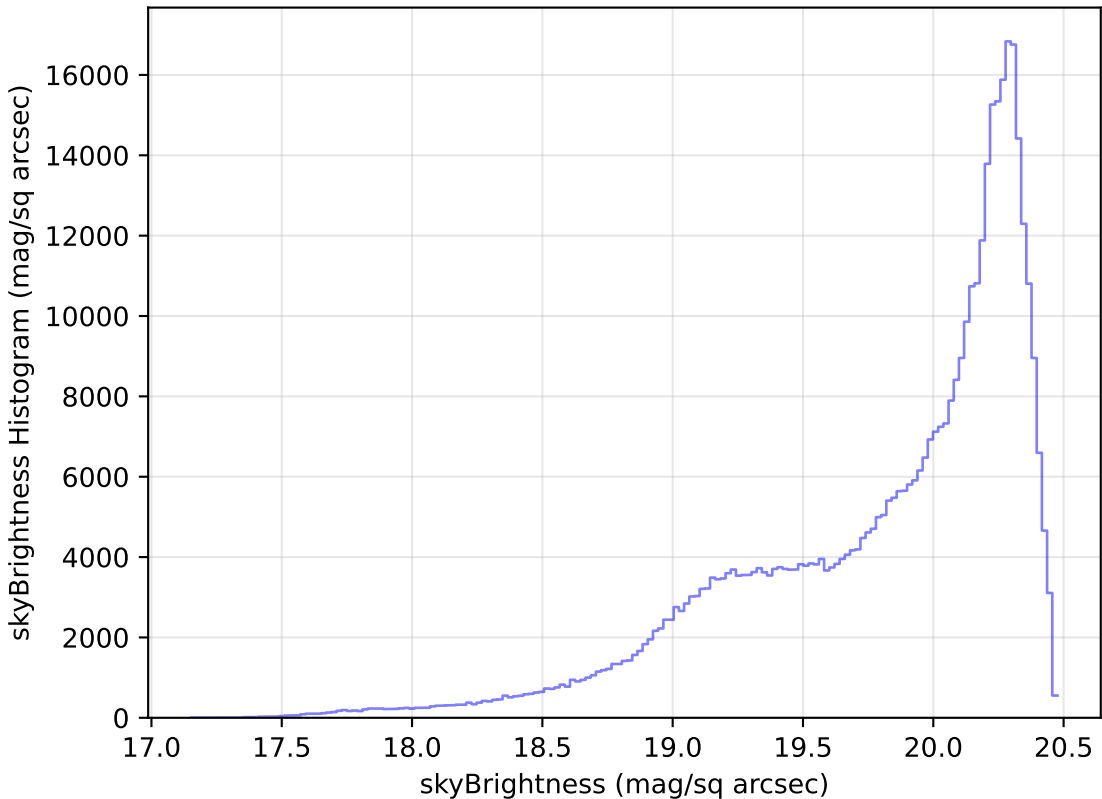
too_100_4v3.4_10yrs All sky i band: skyBrightness Histogram
