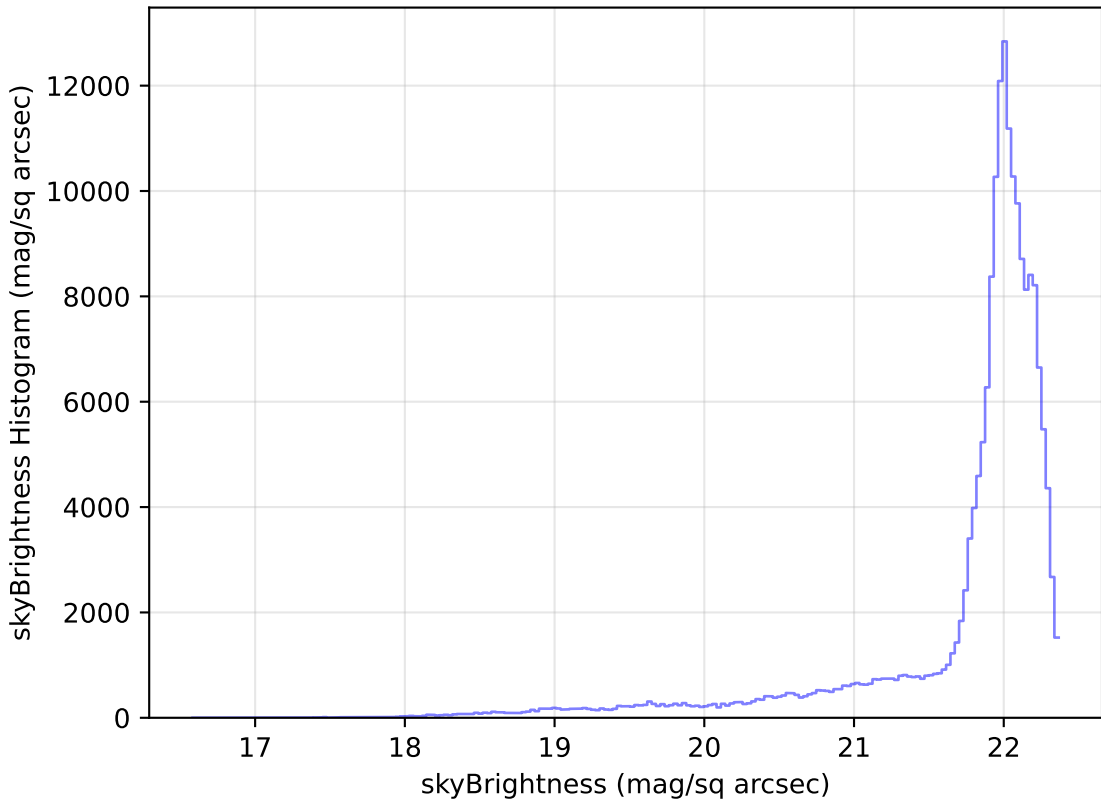
too_100_4v3.4_10yrs All sky g band: skyBrightness Histogram
