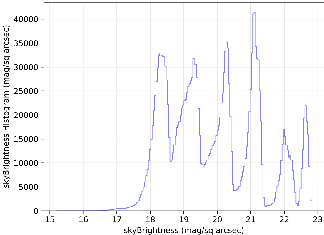
too_100_4v3.4_10yrs All sky all bands: skyBrightness Histogram
