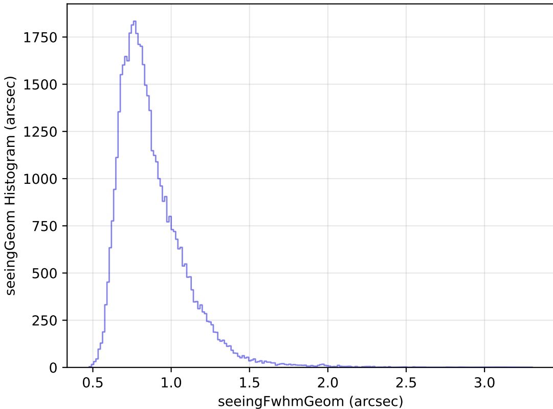
too_100_4v3.4_10yrs Yr 1 y band: seeingGeom Histogram
