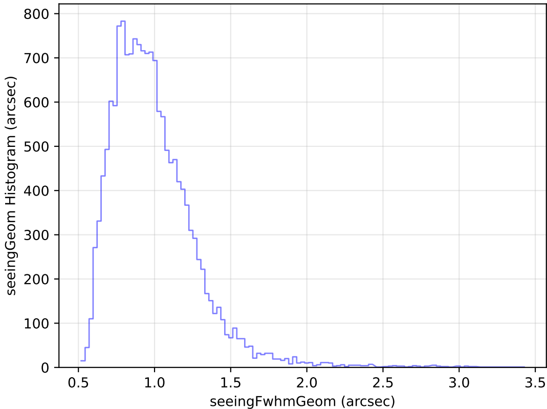
too_100_4v3.4_10yrs Yr 1 u band: seeingGeom Histogram
