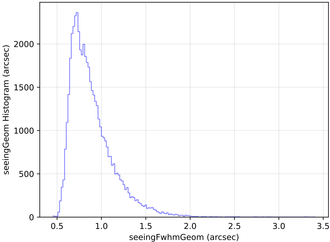
too_100_4v3.4_10yrs Yr 1 r band: seeingGeom Histogram
