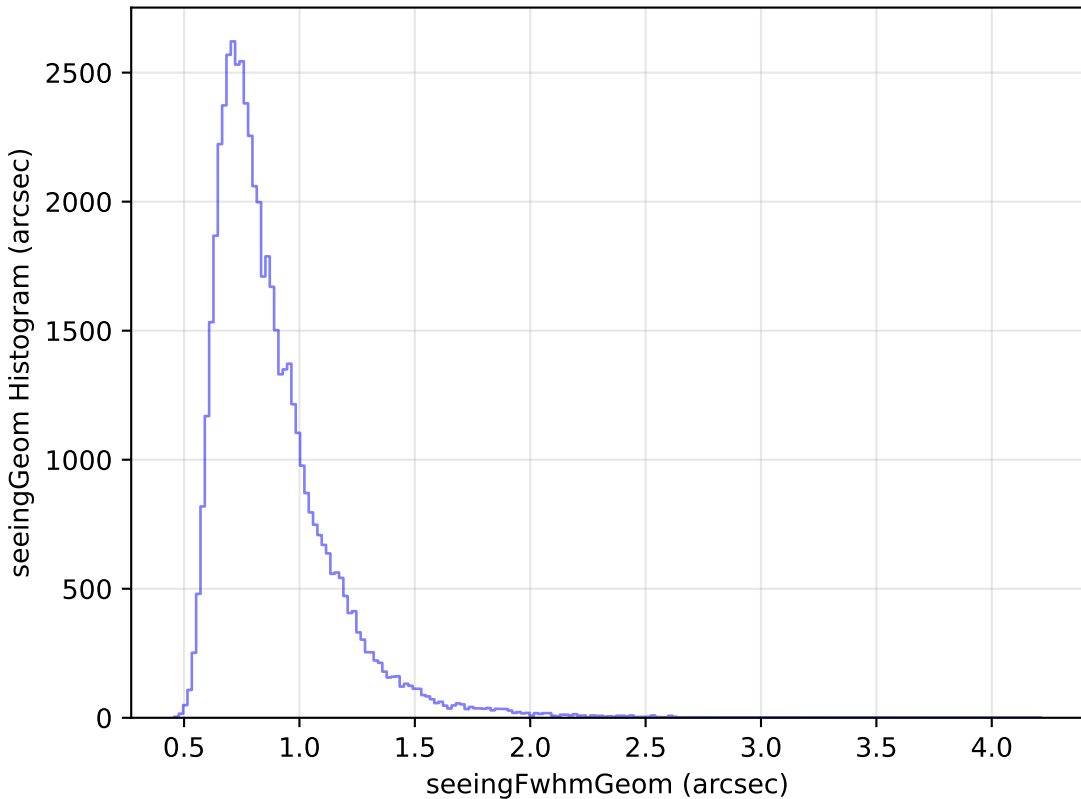
too_100_4v3.4_10yrs Yr 1 i band: seeingGeom Histogram
