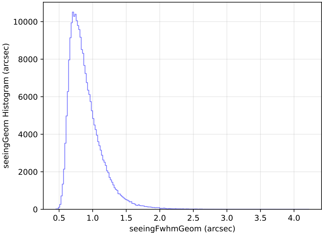
too_100_4v3.4_10yrs Yr 1 all bands: seeingGeom Histogram
