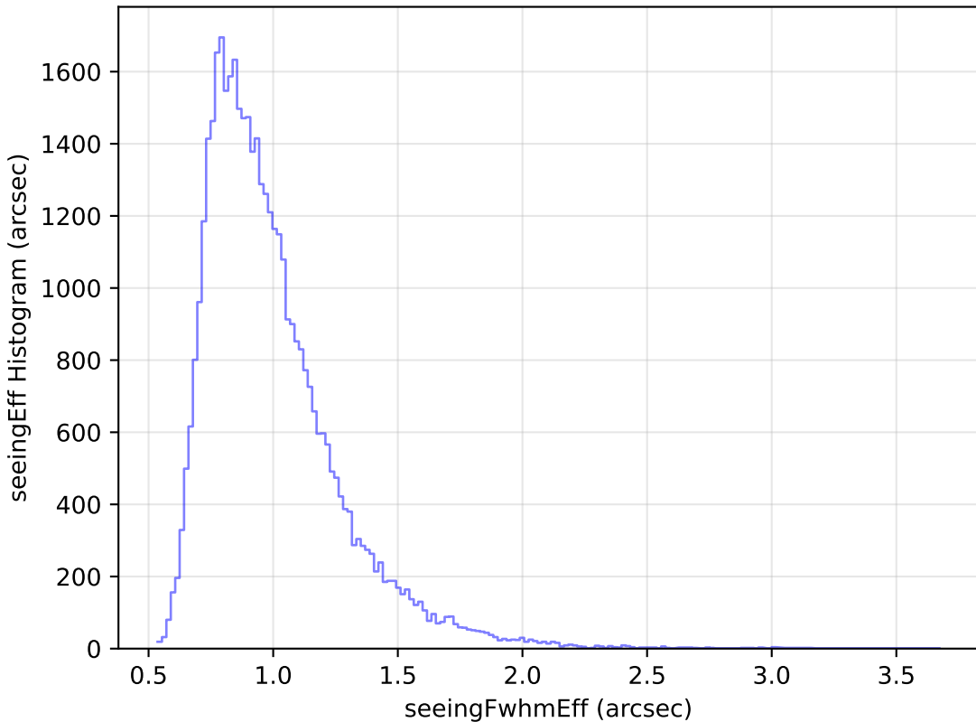
too_100_4v3.4_10yrs Yr 1 z band: seeingEff Histogram
