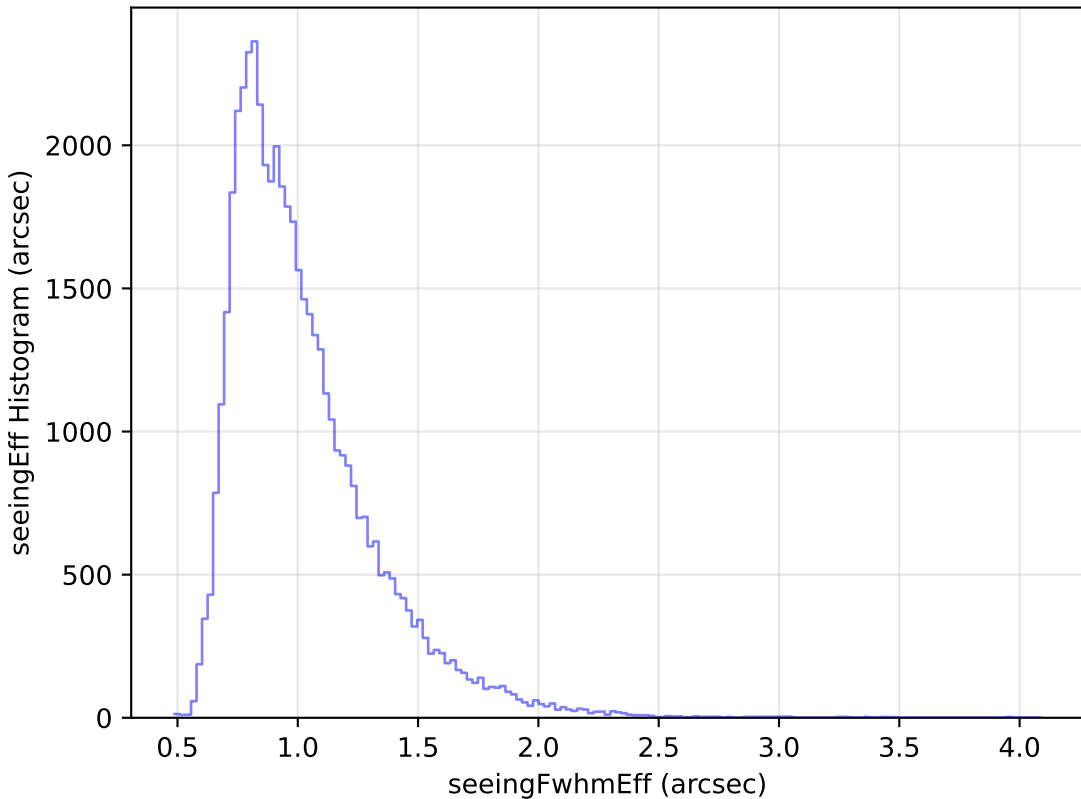
too_100_4v3.4_10yrs Yr 1 r band: seeingEff Histogram
