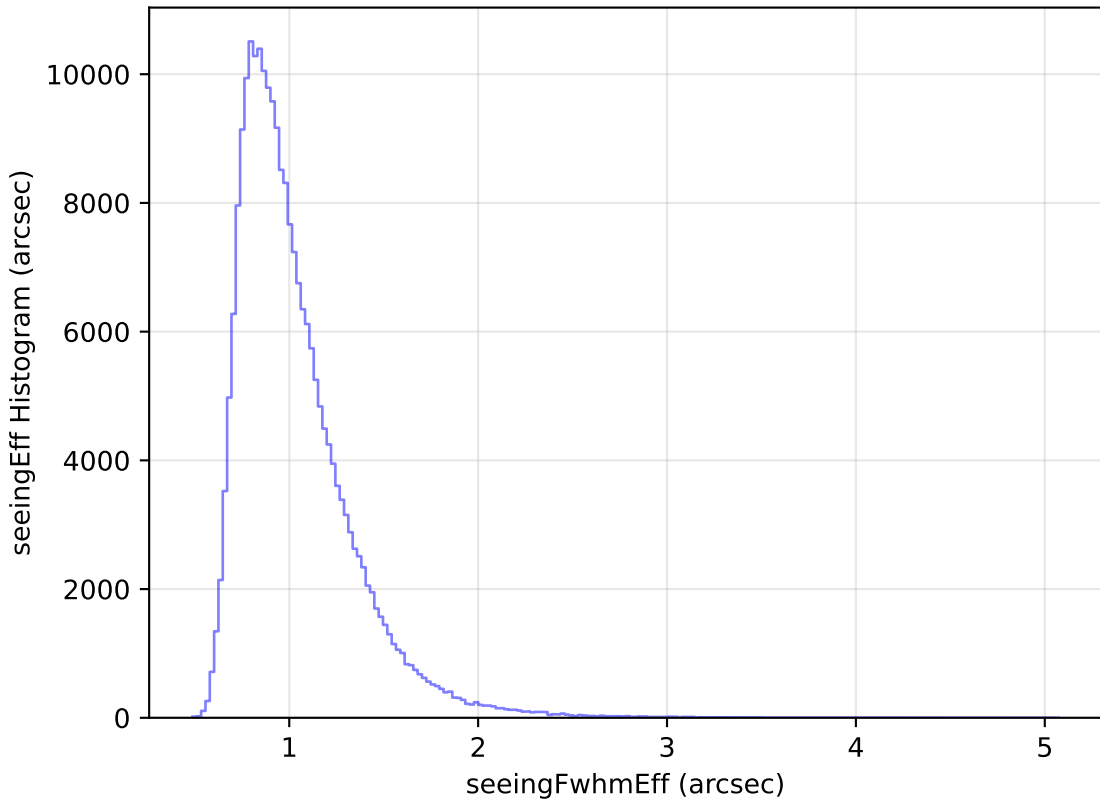
too_100_4v3.4_10yrs Yr 1 all bands: seeingEff Histogram
