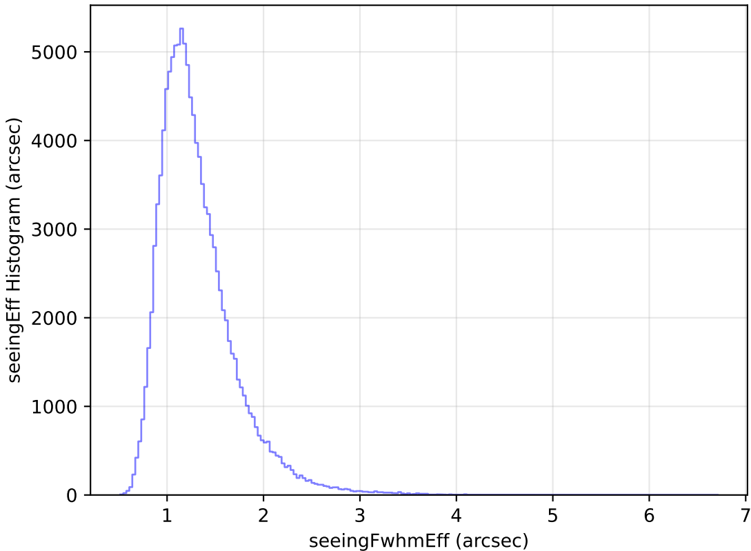
too_100_4v3.4_10yrs WFD u band: seeingEff Histogram
