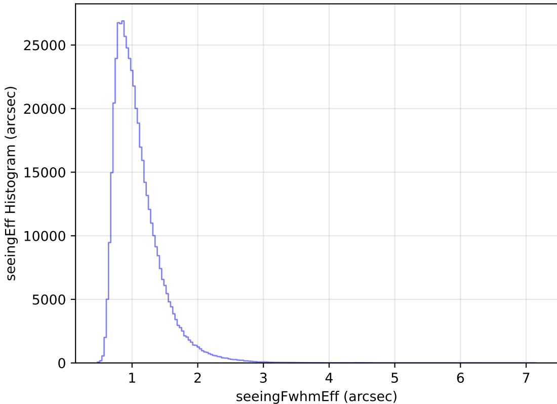
too_100_4v3.4_10yrs WFD i band: seeingEff Histogram
