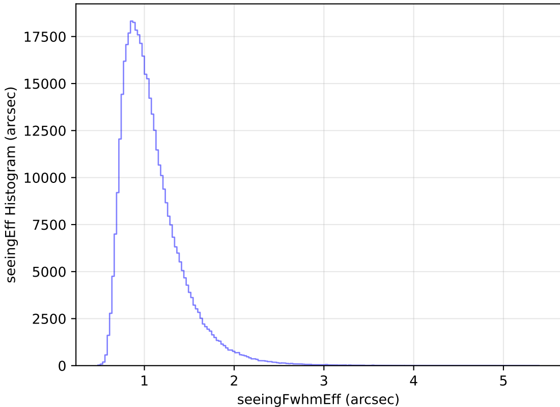
too_100_4v3.4_10yrs All sky z band: seeingEff Histogram
