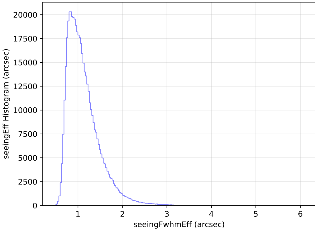
too_100_4v3.4_10yrs All sky r band: seeingEff Histogram
