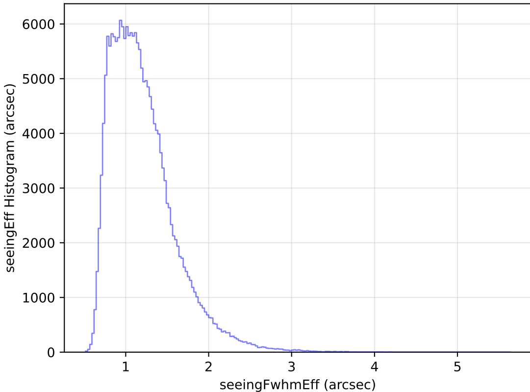
too_100_4v3.4_10yrs All sky g band: seeingEff Histogram
