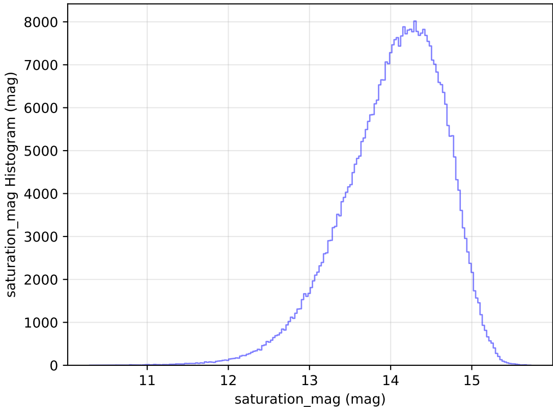
too_100_4v3.4_10yrs WFD z band: saturation_mag Histogram
