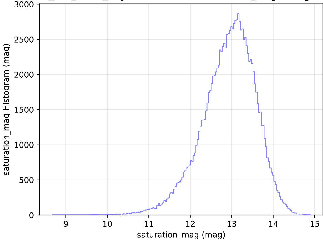
too_100_4v3.4_10yrs WFD u band: saturation_mag Histogram
