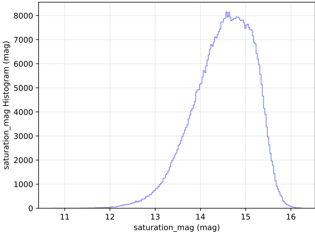
too_100_4v3.4_10yrs WFD r band: saturation_mag Histogram
