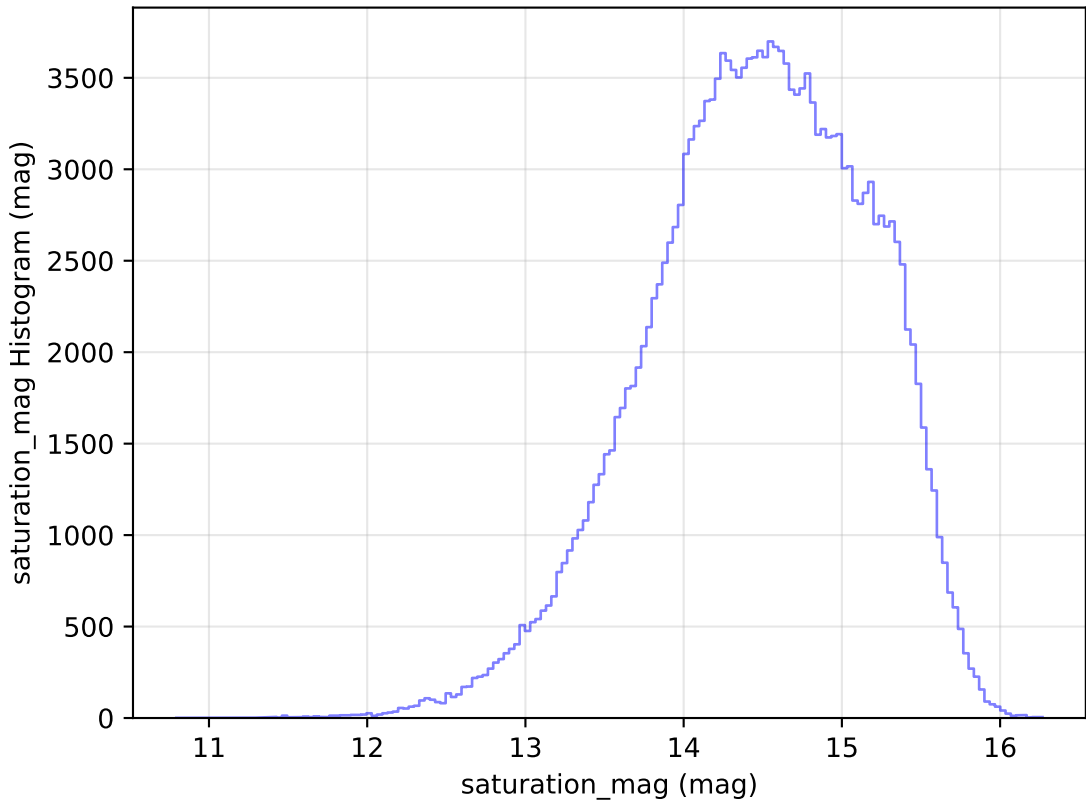
too_100_4v3.4_10yrs WFD g band: saturation_mag Histogram
