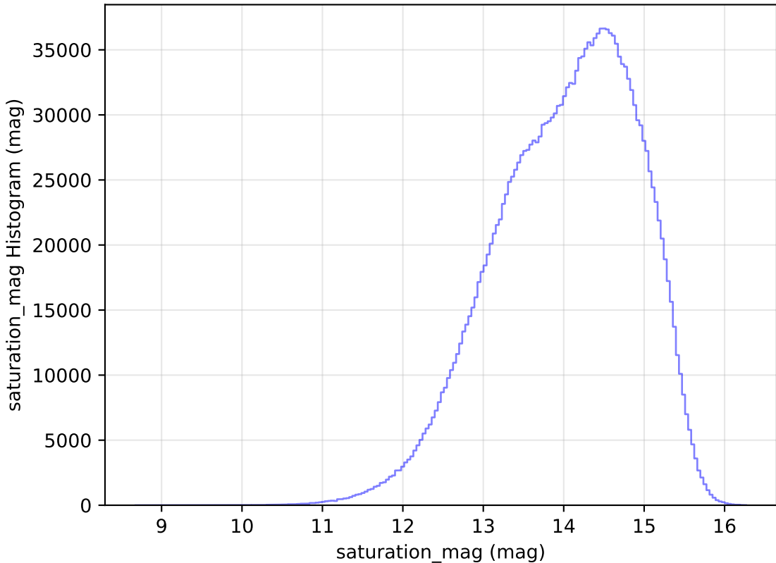
too_100_4v3.4_10yrs WFD all bands: saturation_mag Histogram
