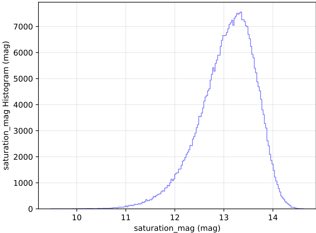
too_100_4v3.4_10yrs All sky y band: saturation_mag Histogram
