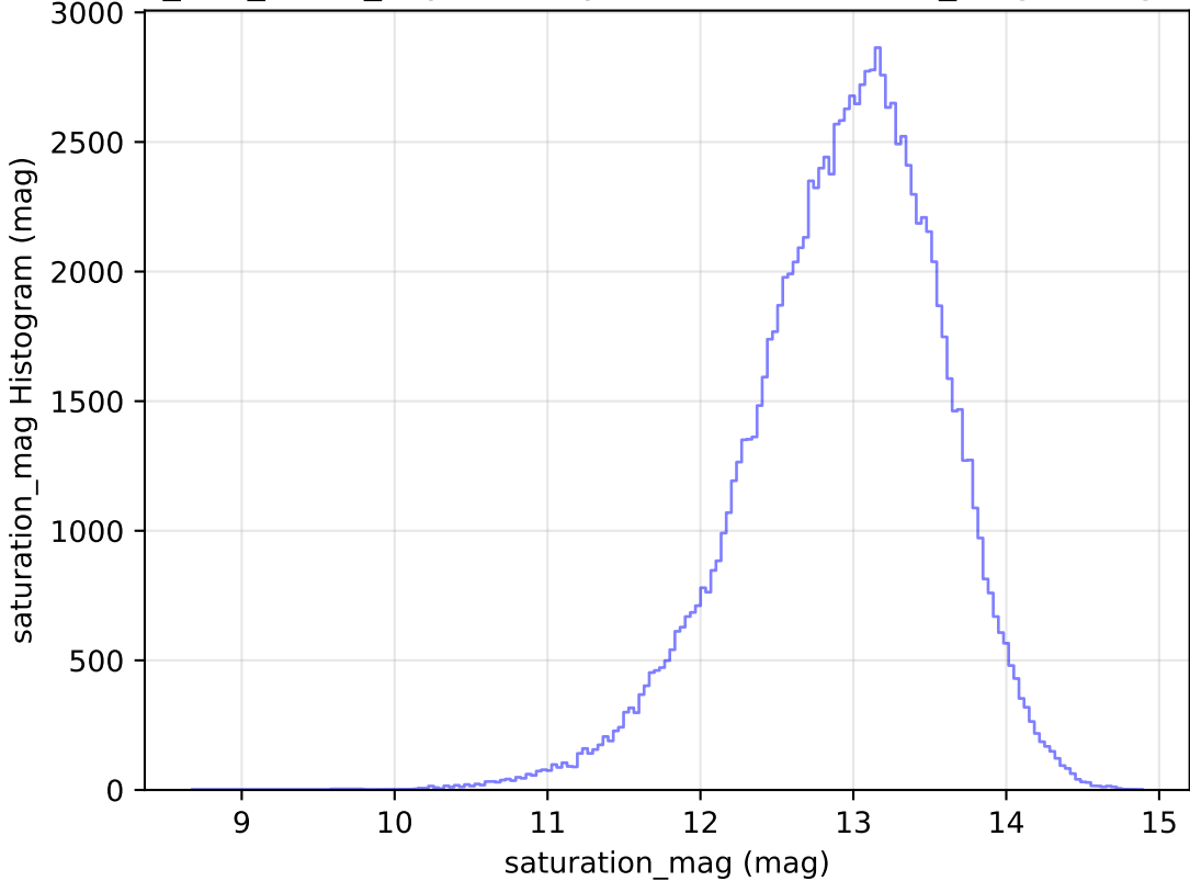
too_100_4v3.4_10yrs All sky u band: saturation_mag Histogram
