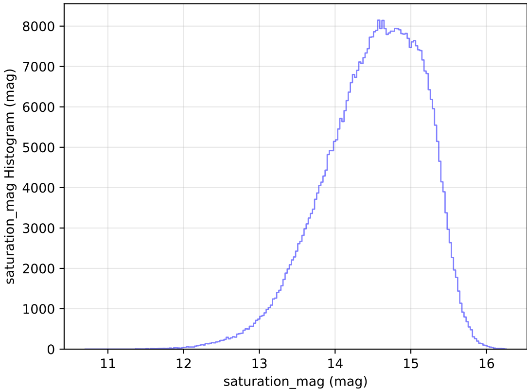
too_100_4v3.4_10yrs All sky r band: saturation_mag Histogram
