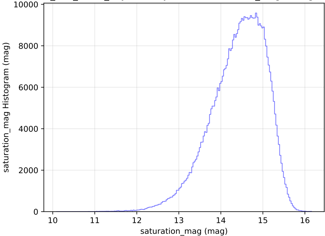
too_100_4v3.4_10yrs All sky i band: saturation_mag Histogram
