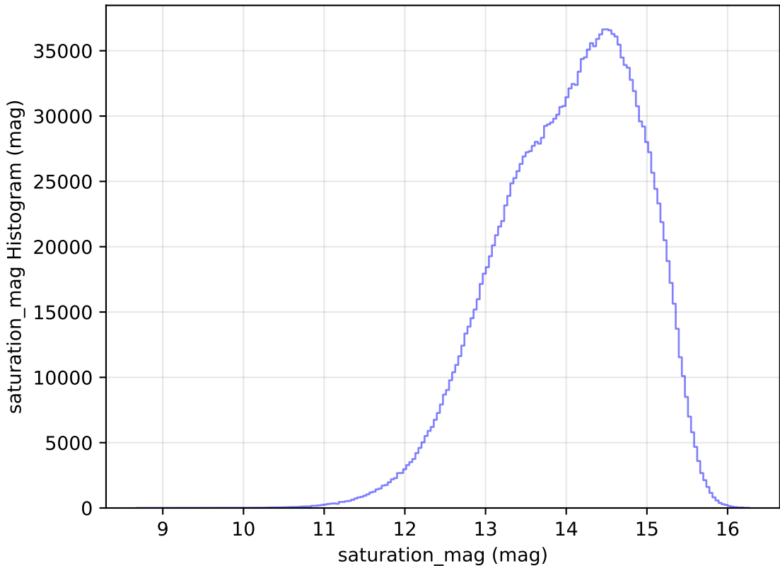
too_100_4v3.4_10yrs All sky all bands: saturation_mag Histogram
