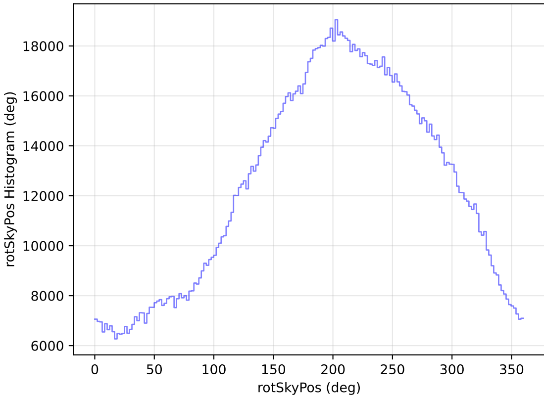
too_100_4v3.4_10yrs WFD all bands: rotSkyPos Histogram
