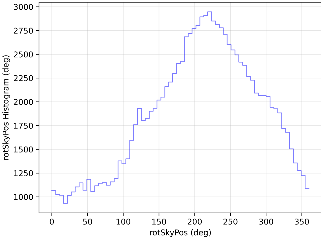
too_100_4v3.4_10yrs All sky u band: rotSkyPos Histogram
