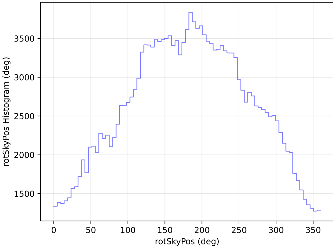
too_100_4v3.4_10yrs All sky g band: rotSkyPos Histogram
