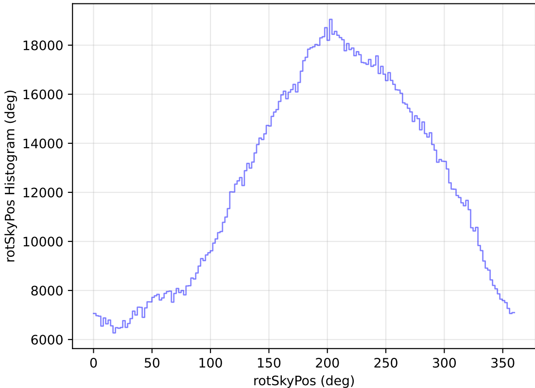
too_100_4v3.4_10yrs All sky all bands: rotSkyPos Histogram
