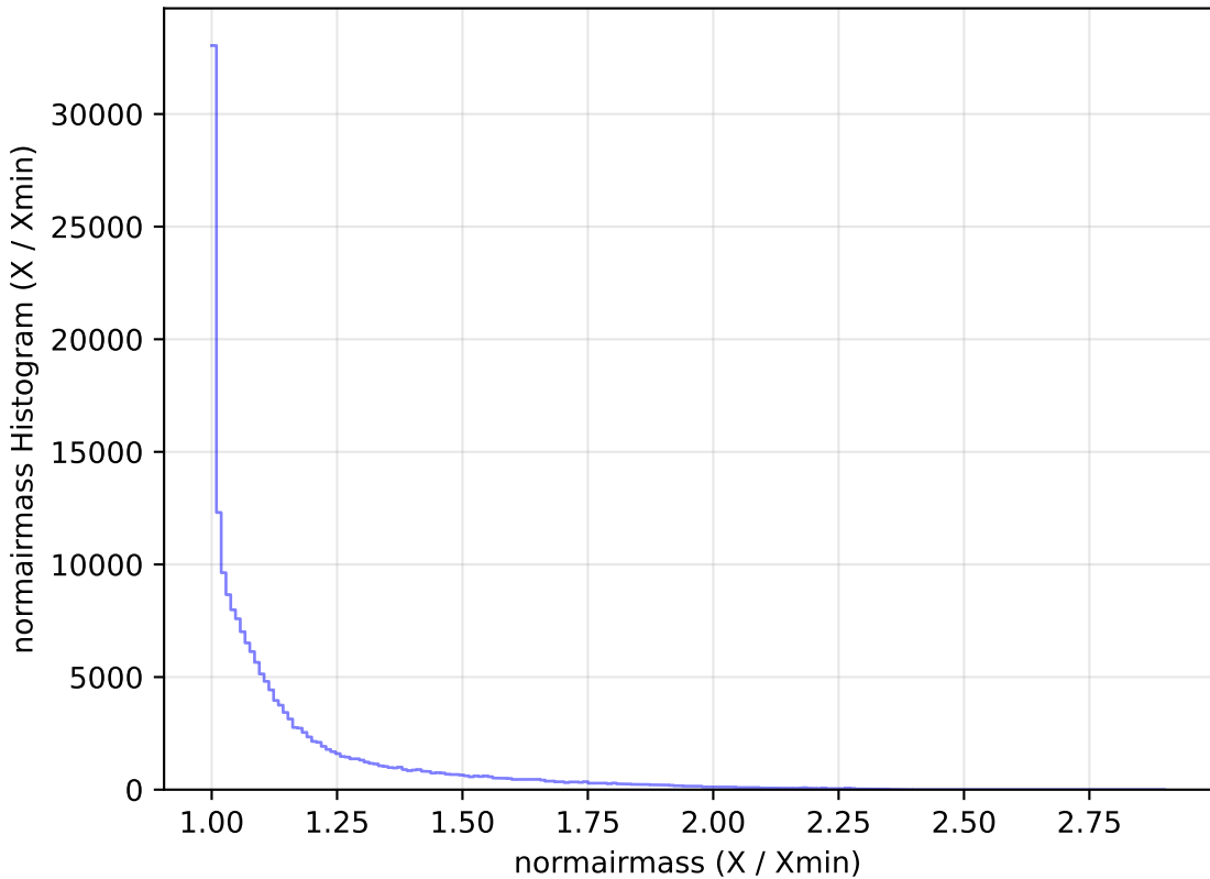
too_100_4v3.4_10yrs WFD g band: normairmass Histogram
