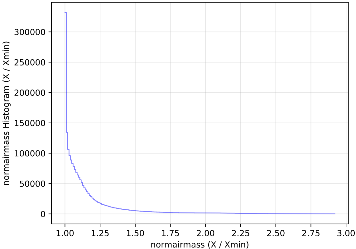
too_100_4v3.4_10yrs WFD all bands: normairmass Histogram
