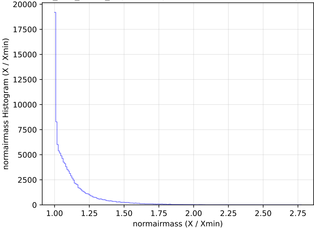
too_100_4v3.4_10yrs All sky u band: normairmass Histogram
