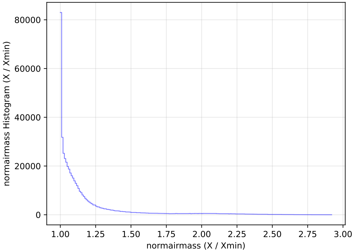
too_100_4v3.4_10yrs All sky i band: normairmass Histogram
