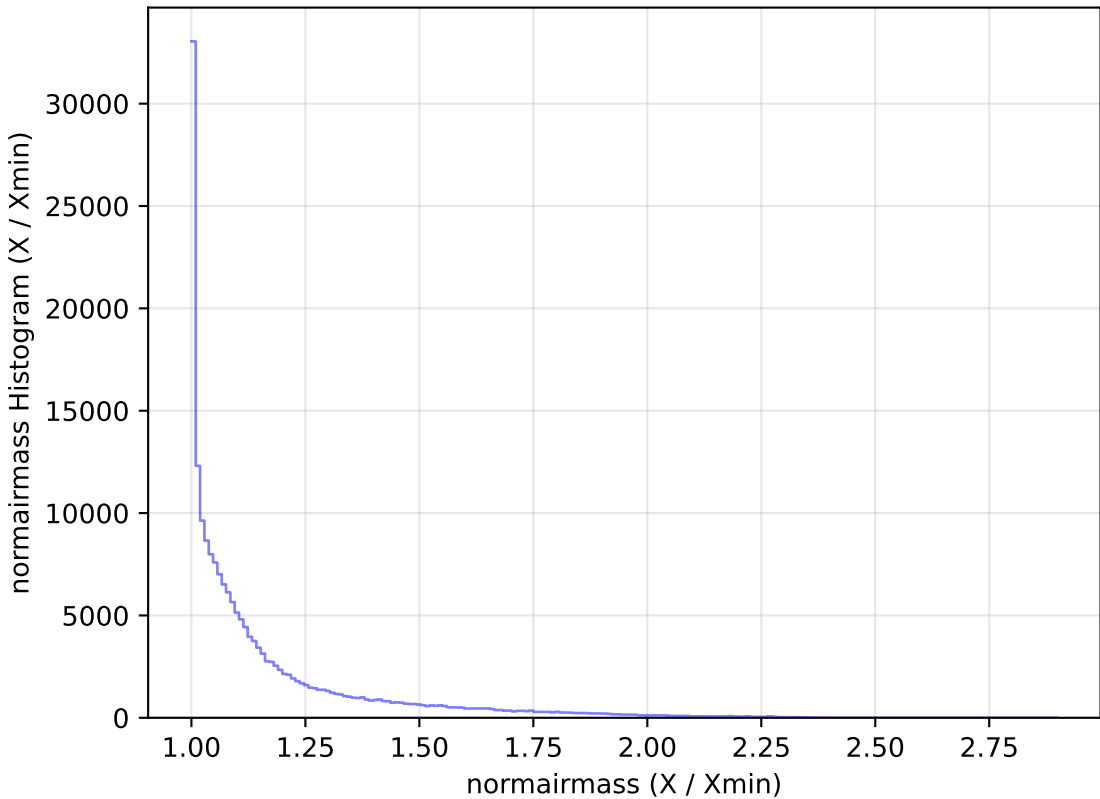
too_100_4v3.4_10yrs All sky g band: normairmass Histogram
