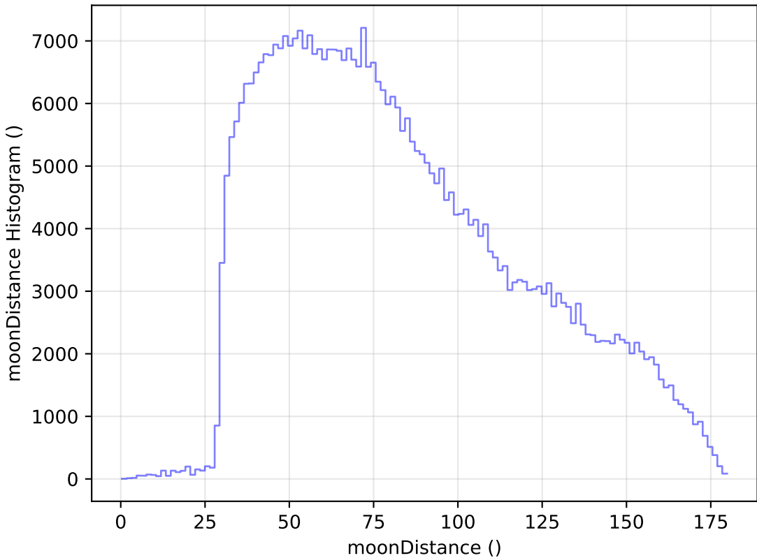
too_100_4v3.4_10yrs WFD z band: moonDistance Histogram
