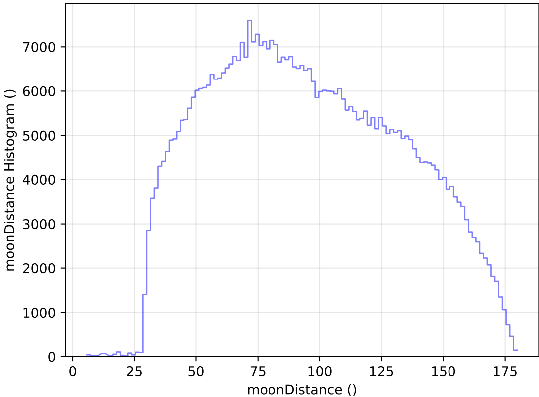
too_100_4v3.4_10yrs WFD i band: moonDistance Histogram
