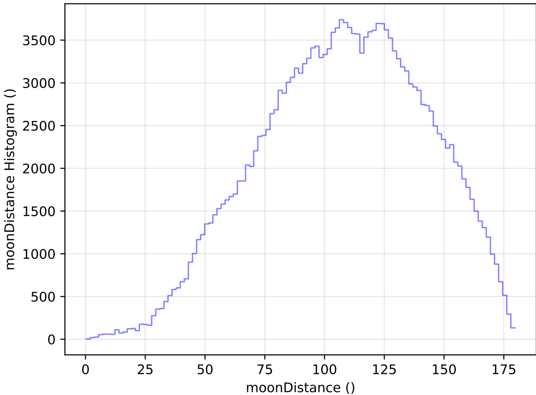
too_100_4v3.4_10yrs WFD g band: moonDistance Histogram
