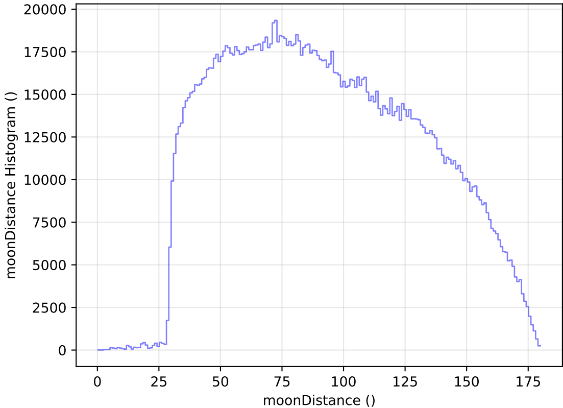
too_100_4v3.4_10yrs WFD all bands: moonDistance Histogram
