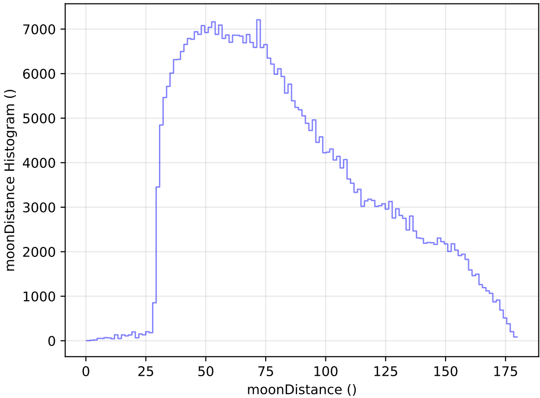
too_100_4v3.4_10yrs All sky z band: moonDistance Histogram
