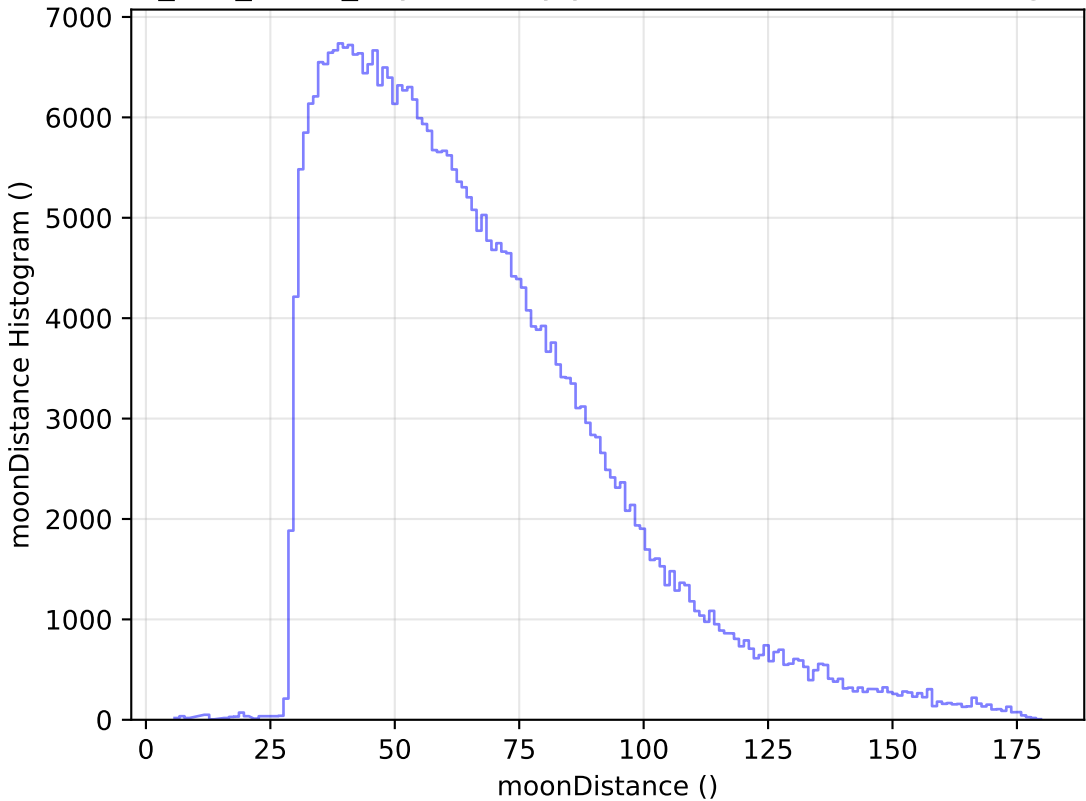
too_100_4v3.4_10yrs All sky y band: moonDistance Histogram
