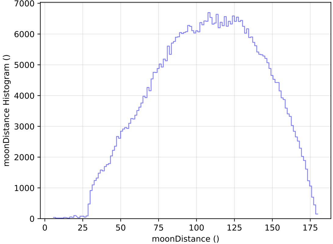
too_100_4v3.4_10yrs All sky r band: moonDistance Histogram
