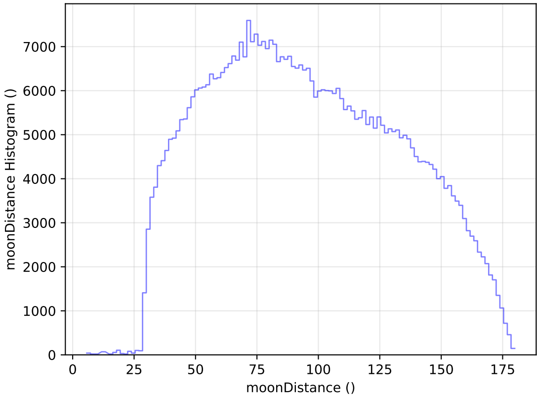
too_100_4v3.4_10yrs All sky i band: moonDistance Histogram
