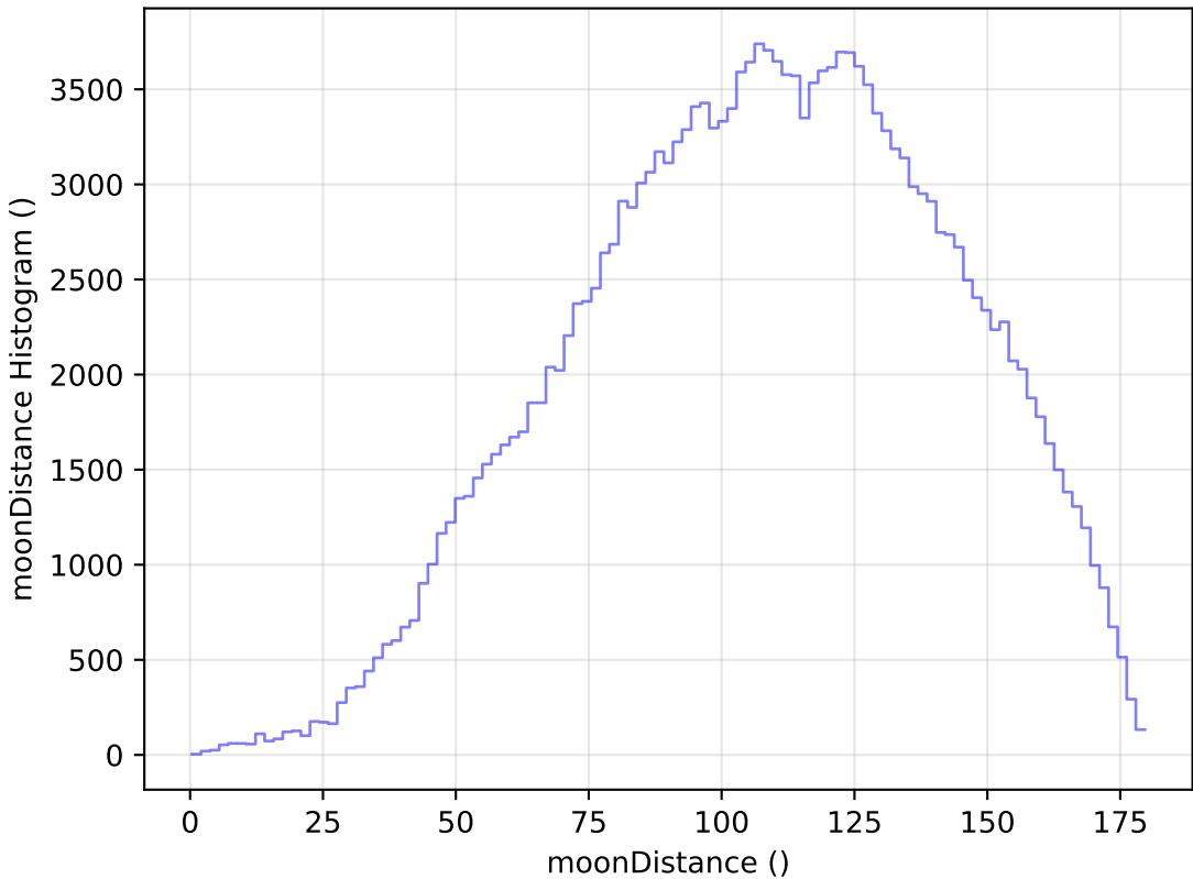
too_100_4v3.4_10yrs All sky g band: moonDistance Histogram
