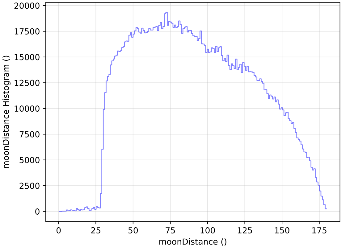
too_100_4v3.4_10yrs All sky all bands: moonDistance Histogram
